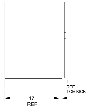
Side View Recessed Base
